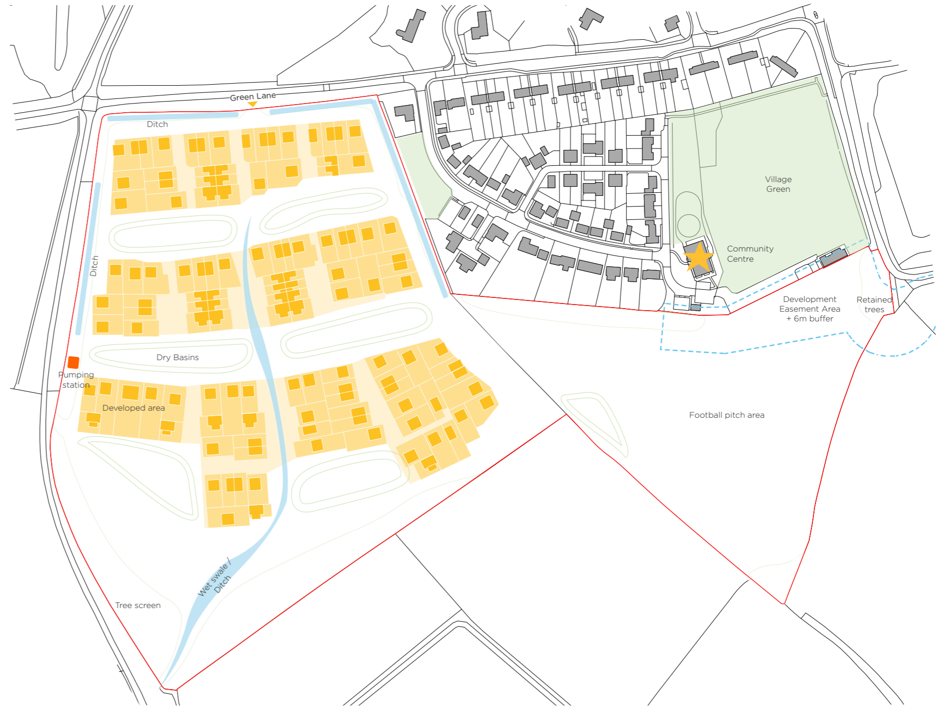
01 Site drainage strategy
